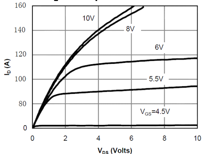
Figure3. Output Characteristics
