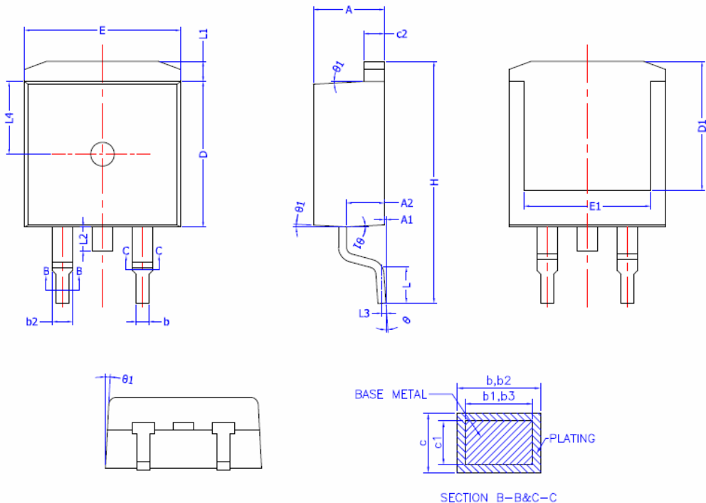
SECTION B-B&amp;C-C
