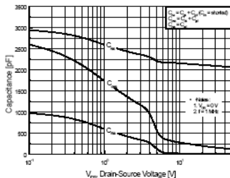
Figure 5. Capacitance Characteristics
