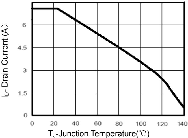
Figure 4 Drain Current
