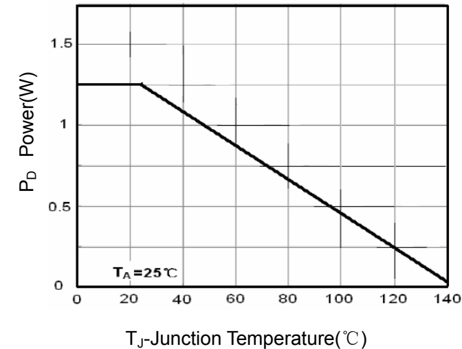
Figure 3 Power Dissipation
