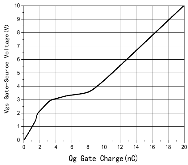
Fig6 Gate Charge
