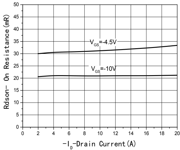
Fig3 Rdson-Drain current
