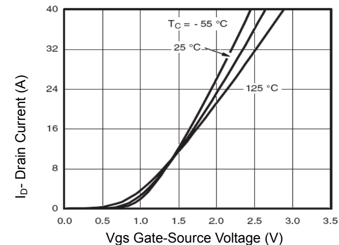
Figure 7 Transfer Characteristics
