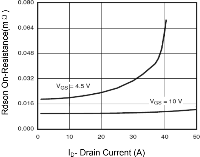
Figure 6 Drain-Source On-Resistance
