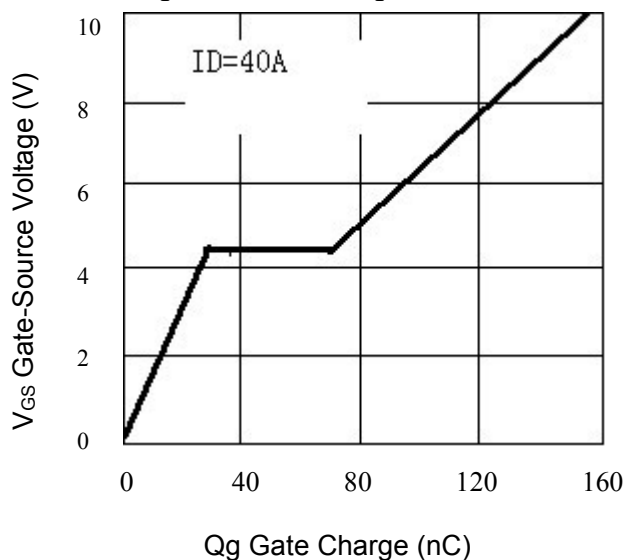
Figure5. Gate Charge
